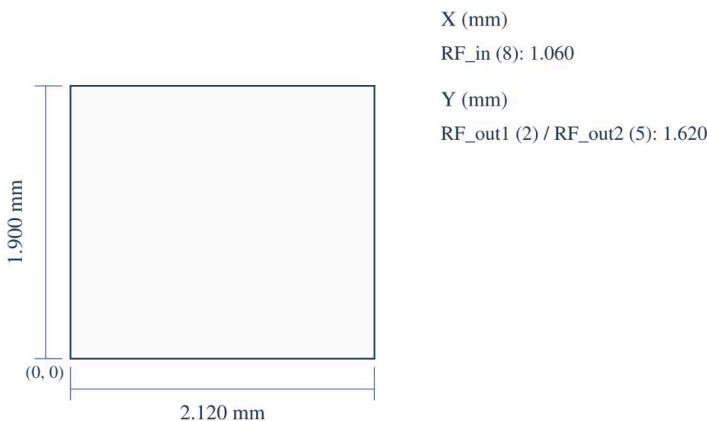
LCDIV-2000-18000-2WAY-D-S2p12X1p9
